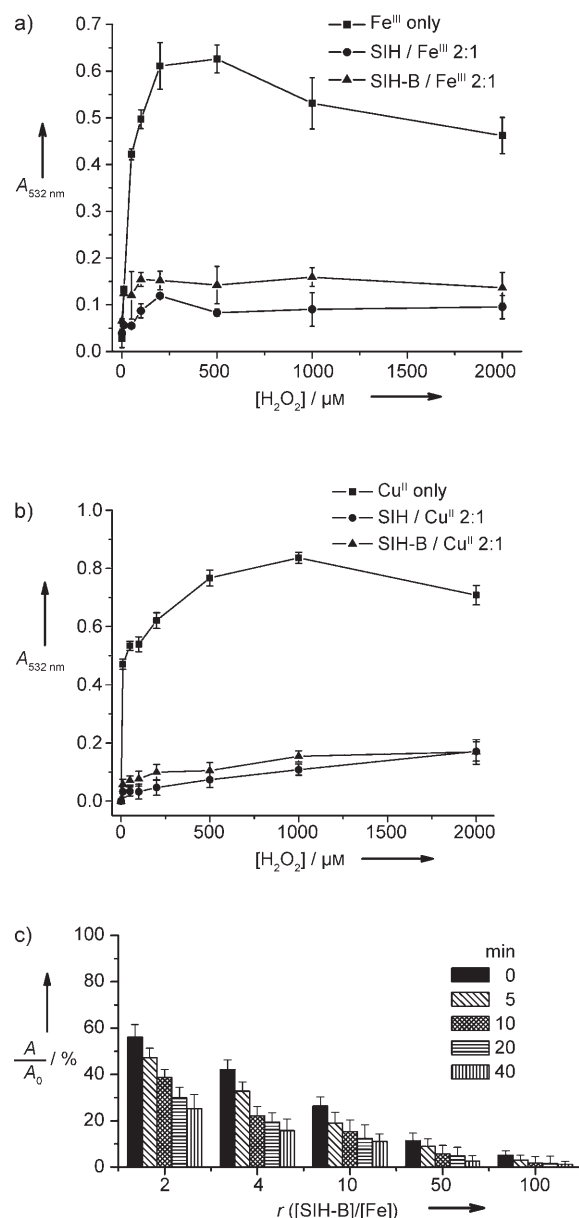
Figure 3. Effect of SIH and SIH-B on the oxidative degradation of 2-deoxyribose promoted by a) Fe III or b) Cu II in the presence of \text{H}_2\text{O}_2 and hydroascorbate. SIH-B (50 \mu\text{M} ) was preincubated with \text{H}_2\text{O}_2 for 45 min at 298 K, then the solution (0.5 mL) was added to the assay system containing Fe III (or Cu II ; 25 \mu\text{M} ), 2-deoxyribose (10 mM), and hydroascorbate (200 \mu\text{M} ) in KPB (20 mM, pH 7.2). c) Effect of preincubation time (0, 5, 10, 20, 40 min) and [\text{SIH-B}]/[\text{Fe}] ratio ( r ) on attenuation of Fe II -promoted Fenton chemistry in KPB buffer (20 mM, pH 7.2). [\text{Fe}] = 10 \mu\text{M} , [\text{H}_2\text{O}_2] = 200 \mu\text{M} ; A and A_0 are the absorbance at 532 nm in the presence and absence of SIH-B, respectively.
